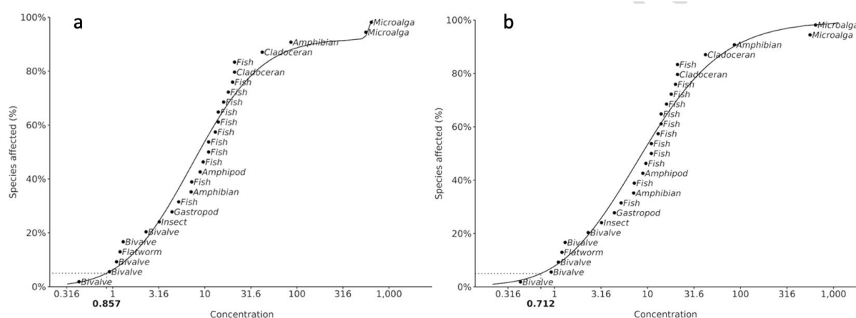
Figure C.2 Species sensitivity distribution for dataset B (n = 27) (a) using the full default model set and (b) without l-norm–l-norm in the model set
